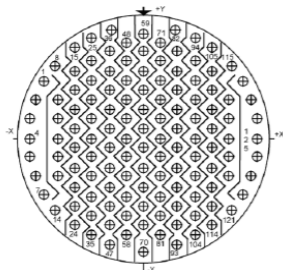
Contact Layout
