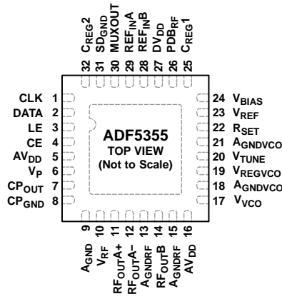
Figure 3. Pin Configuration
