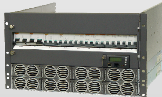
16 kW in 19", 6 RU with Controller, Load & Battery Distribution
