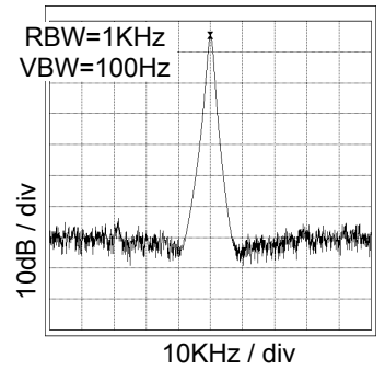
Fig.55 16.9MHz Spectrum VDD=3.3V, at CL=15pF
