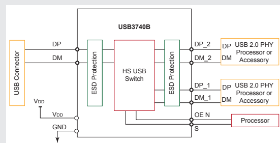
USB Switching Diagram
