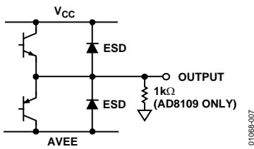
Figure 44. Analog Output
