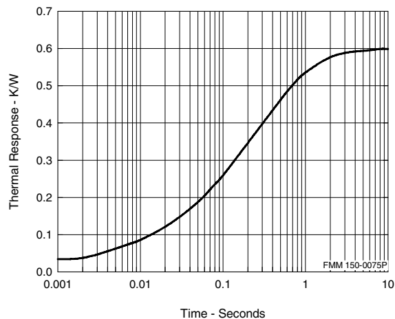
Fig. 18 Therm. impedance junction to case Z_{thJC}
