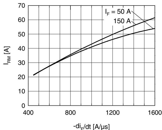
Fig. 14 Reverse recovery current I_{RM} of the body diode vs. di/dt
