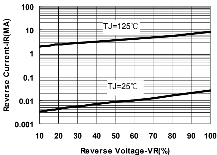
Fig.2-Typical Reverse Characteristics
