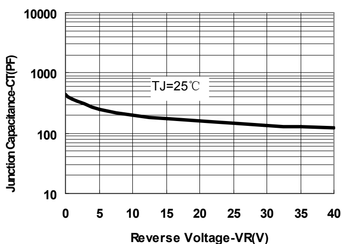
Fig.1-Typical Junction Capacitance
