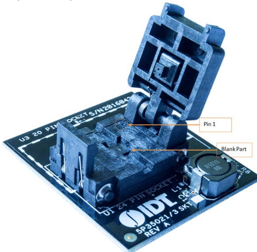
Figure 3. Socket Board (Pin Position)
