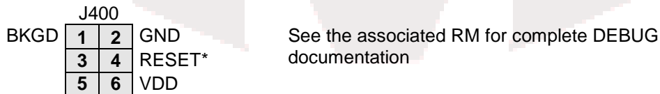
Figure 2: BDM_PORT Header
