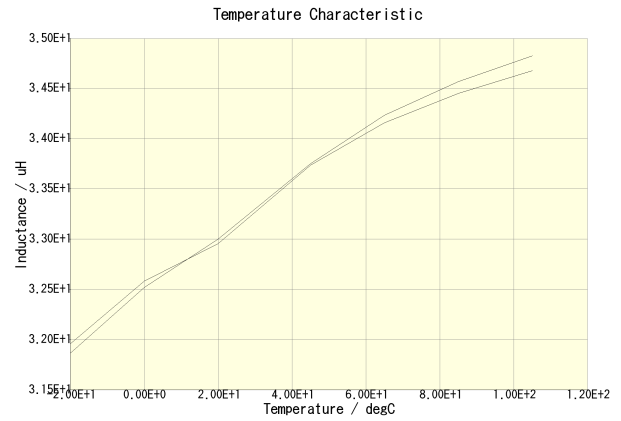
CLF10040T-330M-CA(DC = 0A)
