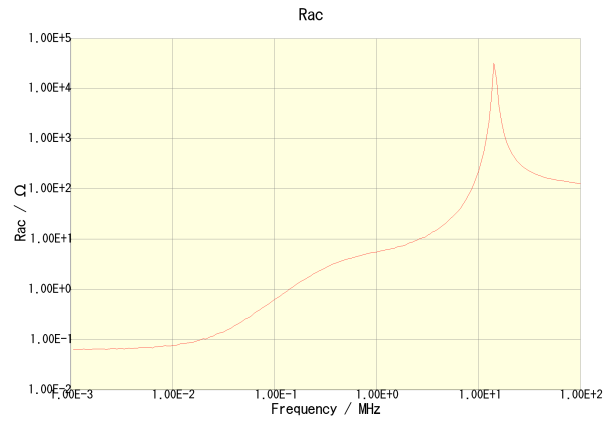
CLF10040T-330M-CA
