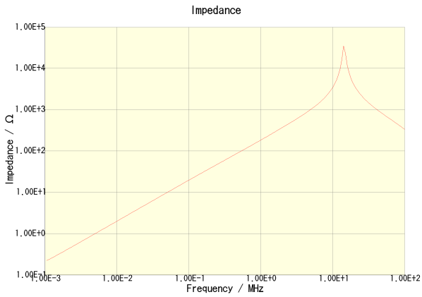
CLF10040T-330M-CA
