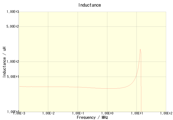
CLF10040T-330M-CA
