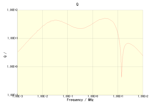
CLF10040T-330M-CA
