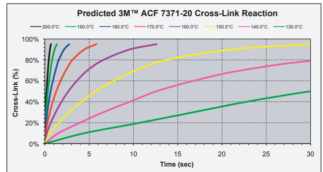
Figure 2. Graph of predicted cross-link reaction compared with bonding temperature and time.
