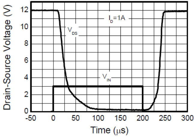
Switching Speed
