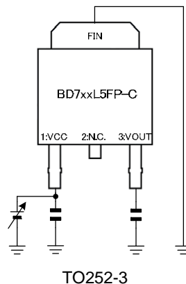
TO252-3 Figure 2. Typical Application Circuits
