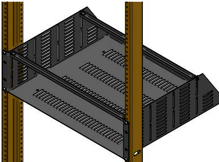
COMPLETE ASSEMBLY
