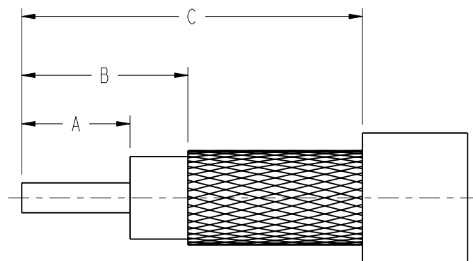
RECOMMENDED CABLE STRIPPING DIM'S (LMR-240)
