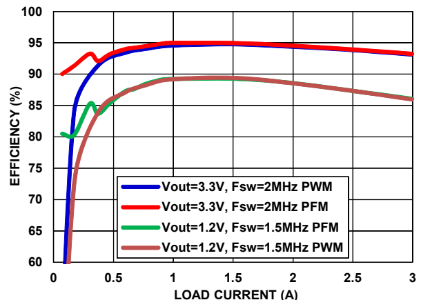
FIGURE 2. EFFICIENCY vs LOAD 5VIN
