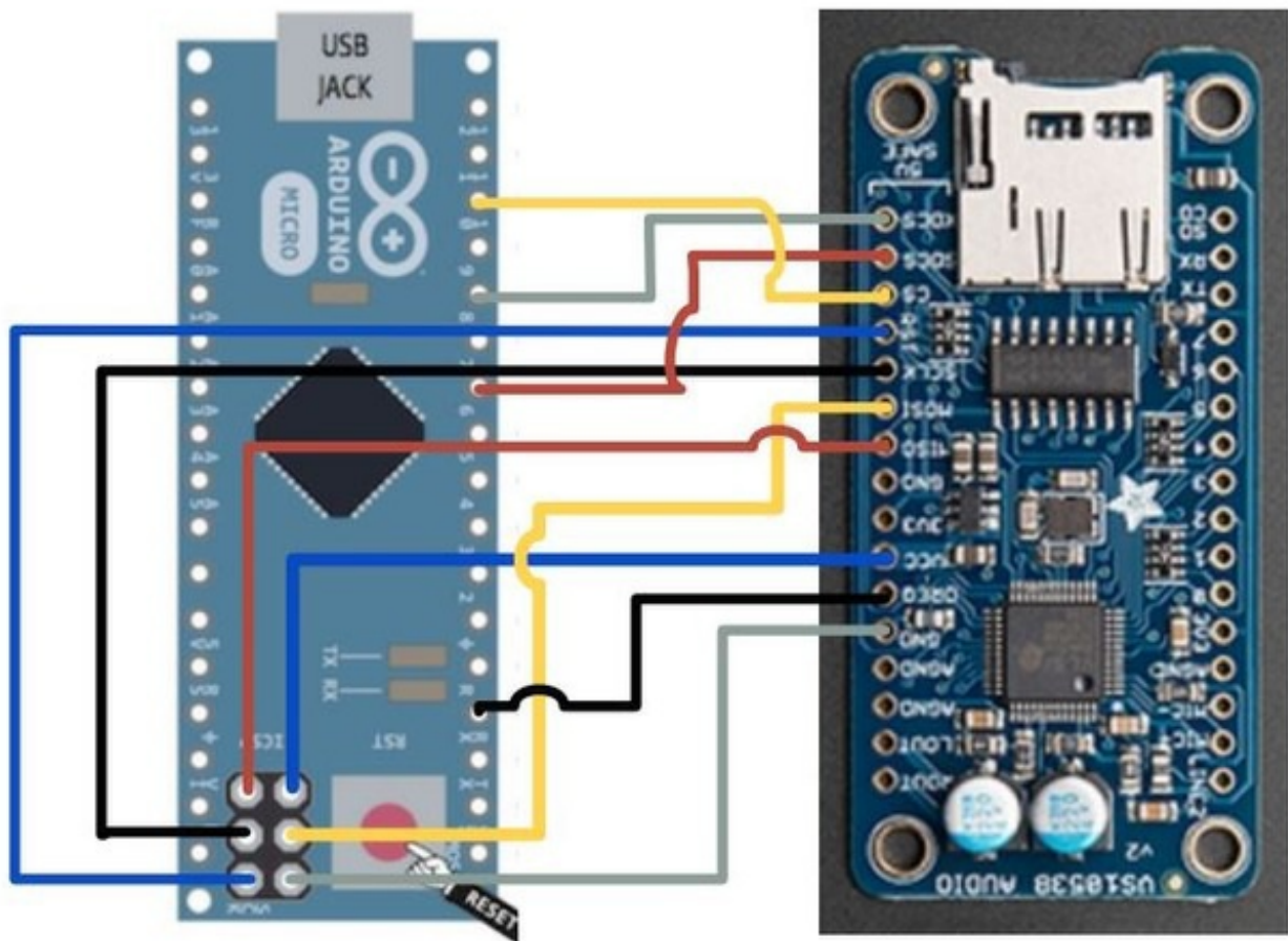
Arduino Micro to Adafruit VS1053 Codec Connections Chart by Frank Cohen, fcohen@votsh.com Distributed Under Creative Commons License February 24, 2014
