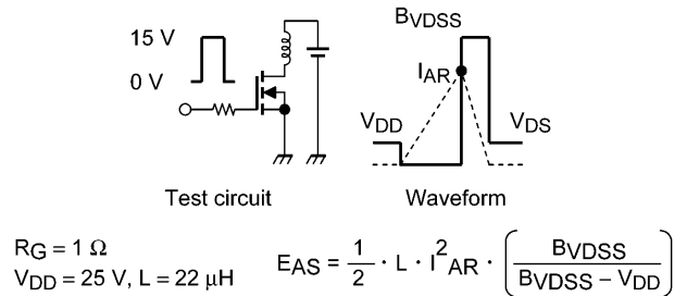
Fig. 8.15 Test Circuit/Waveform
