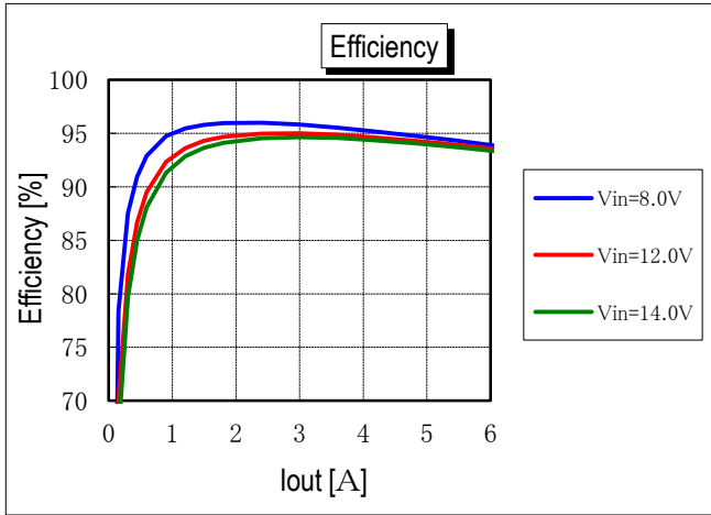
Efficiency vs. Line Voltage and Load Current @ +25° C. (Vout = 3.3V)
