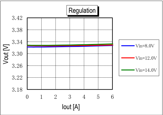
Vout vs. Line Voltage and Load Current @ +25° C. (Vout = 3.3V)
