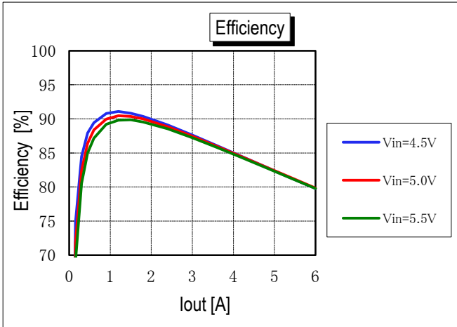
Efficiency vs. Line Voltage and Load Current @ +25° C. (Vout = 0.7V)
