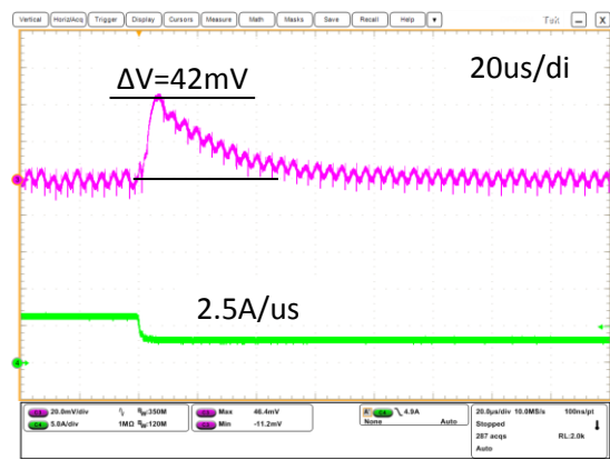
Step Load Transient Response (Vin=5.0V, Vout=0.7V, Cload=400uF, Iout=3A to 6A) Trace 3=Vout, 20 mV/div, Trace 4=Iout, 5A/div.
