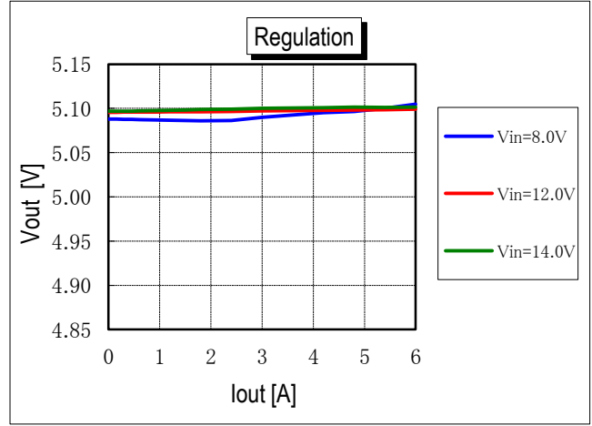
Vout vs. Line Voltage and Load Current @ +25° C. (Vout = 5.0V)
