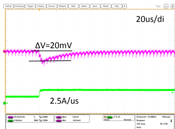
Step Load Transient Response (Vin=5.0V, Vout=1.0V, Cload=400uF, Iout=3A to 6A) Trace 3=Vout, 20 mV/div, Trace 4=Iout, 5A/div.
