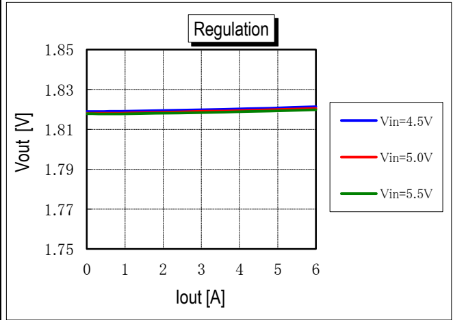
Vout vs. Line Voltage and Load Current @ +25° C. (Vout = 1.8V)
