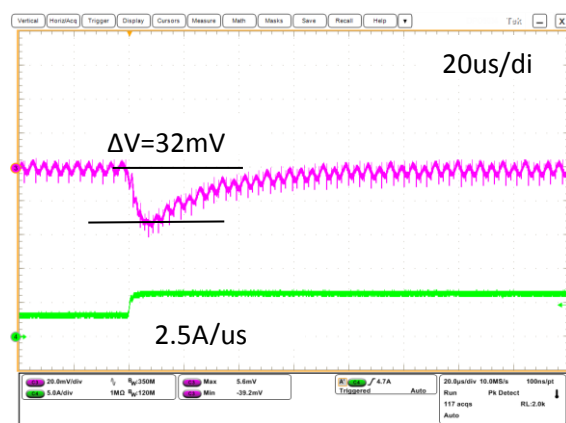
Step Load Transient Response (Vin=5.0V, Vout=1.8V, Cload=400uF, Iout=3A to 6A) Trace 3=Vout, 20 mV/div, Trace 4=Iout, 5A/div.
