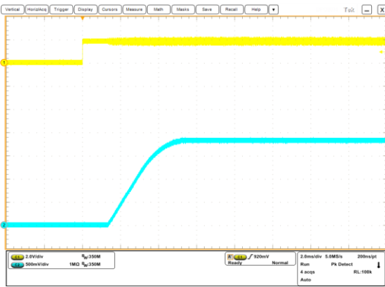
On/Off Enable Delay (Vin=5.0V, Vout=1.8V, Iout=6A, Cload=400uF) Trace1=Enable, Trace2=Vout, 2 ms/div
