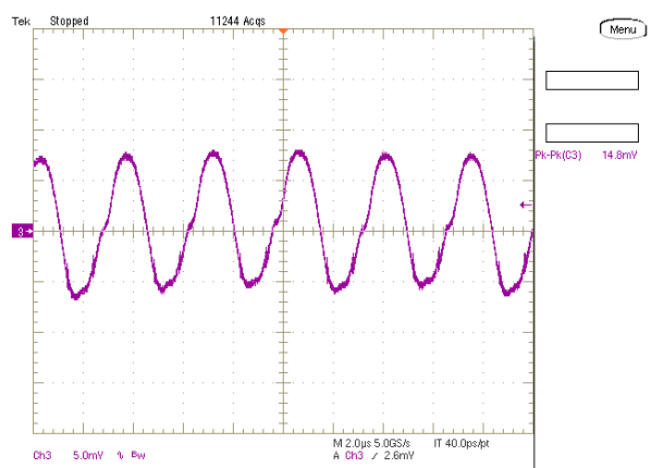
Output Ripple and Noise (Vin=12V, Vout=3.3V, Iout=6A, Cload=400uF, ScopeBW=20MHz)
