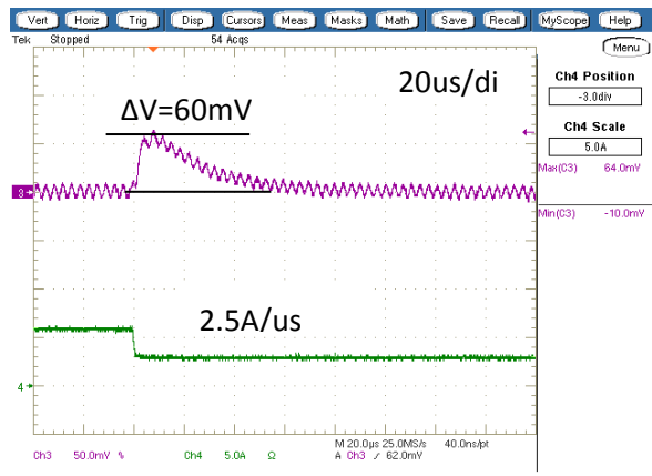
Step Load Transient Response (Vin=12V, Vout=3.3V, Cload=400uF, Iout=3A to 6A) Trace 3=Vout, 50 mV/div, Trace 4=Iout, 5A/div.
