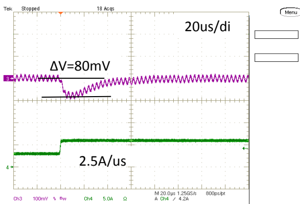
Step Load Transient Response (Vin=12V, Vout=5.0V, Cload=400uF, Iout=3A to 6A) Trace 3=Vout, 100 mV/div, Trace 4=Iout, 5A/div.
