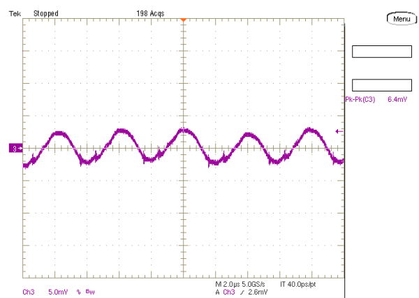
Output Ripple and Noise (Vin=5.0V, Vout=1.0V, Iout=6A, Cload=400uF, ScopeBW=20MHz)
