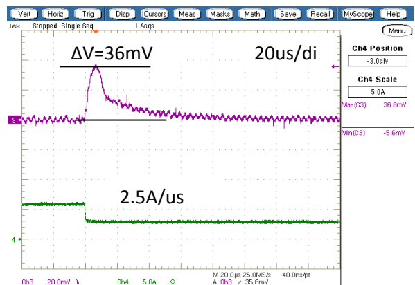
Step Load Transient Response (Vin=12V, Vout=1.0V, Cload=400uF, Iout=3A to 6A) Trace 3=Vout, 20 mV/div, Trace 4=Iout, 5A/div.
