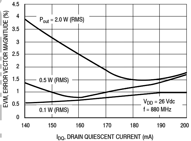
Figure 13. Error Vector Magnitude versus I_{DQ} Total
