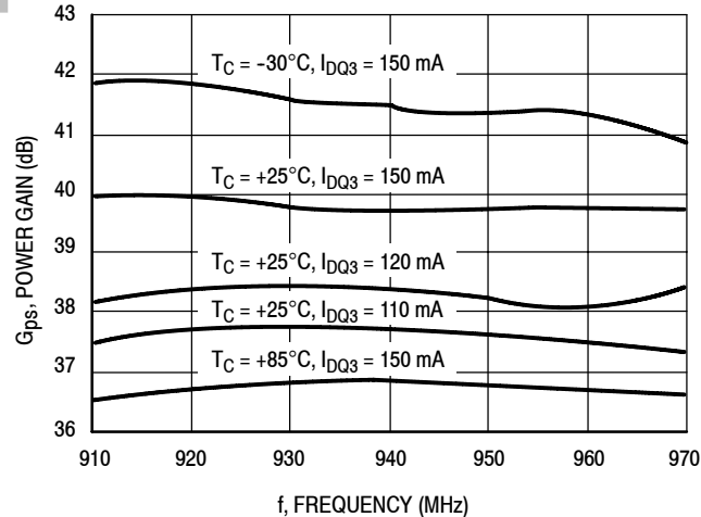
Figure 9. Power Gain versus Frequency P out = P1dB
