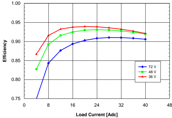
Fig. 3: Efficiency vs. load current and input voltage for converter mounted vertically with air flowing from pin 1 to pin 3 at a rate of 300 LFM (1.5 m/s) and T_a = 25^\circ\text{C} .
