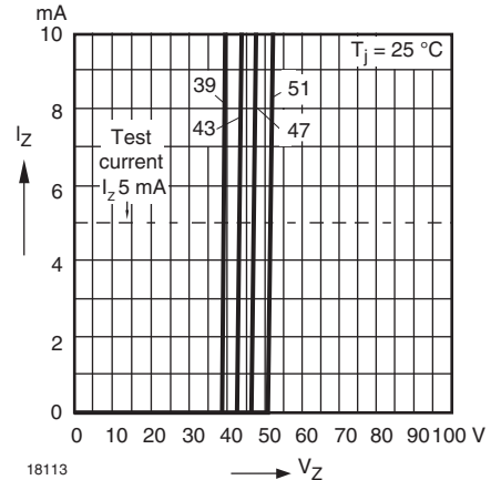
Fig. 16 - Breakdown Characteristics
