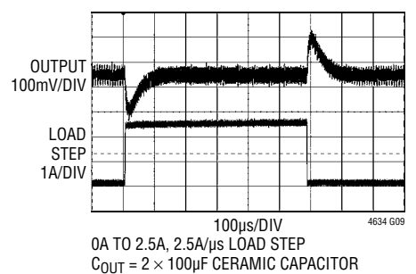
24V to 5V Load Step Response
