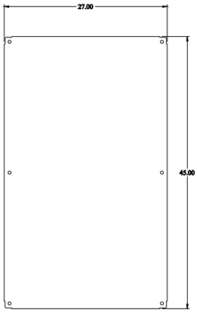
INNER PANEL
