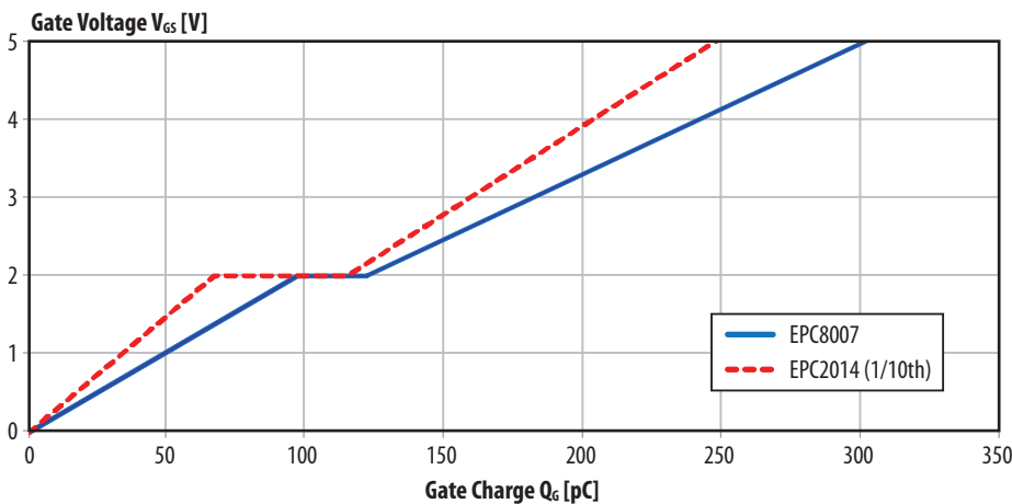
Gate charge of the EPC8007 compared with the EPC2014 scaled to 1/10th of its active area
