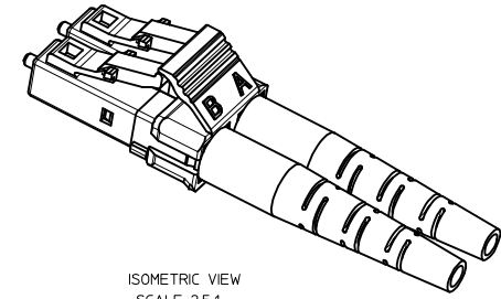
ISOMETRIC VIEW SCALE 2.5:1
