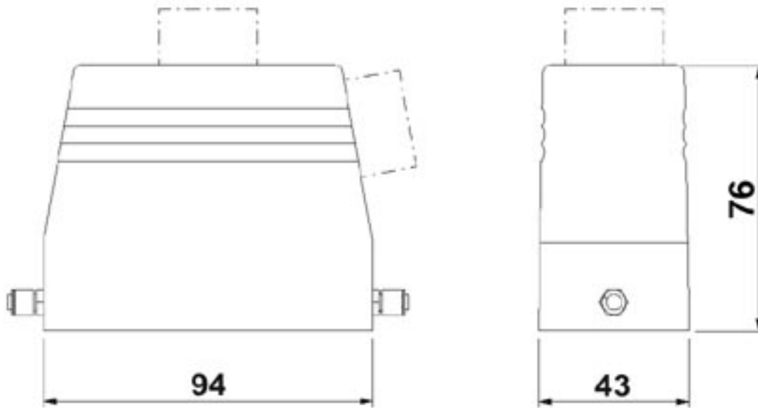
Dimensioned drawing
