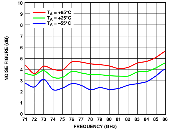
Figure 11. Noise Figure vs. Frequency over Temperature, V_{Dx} = 3 V, I_{Dx} = 50 mA
