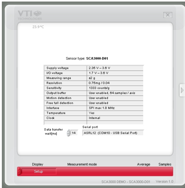
Figure 12. Setup display.
