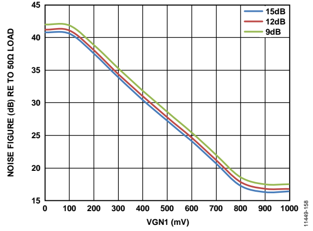
Figure 56. Noise Figure vs. VGN1 over Digital Gain
