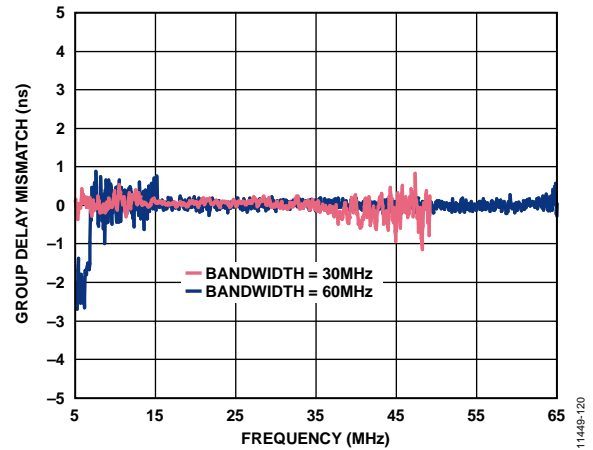
Figure 21. IQ Group Delay Mismatch vs. Frequency (BW = 30 MHz and BW = 60 MHz)
