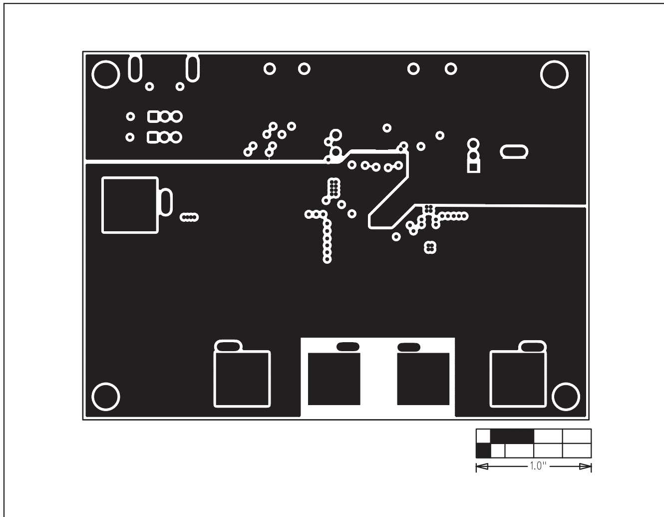
Figure 4. MAX15023 EV Kit PCB Layout—GND Layer 2
