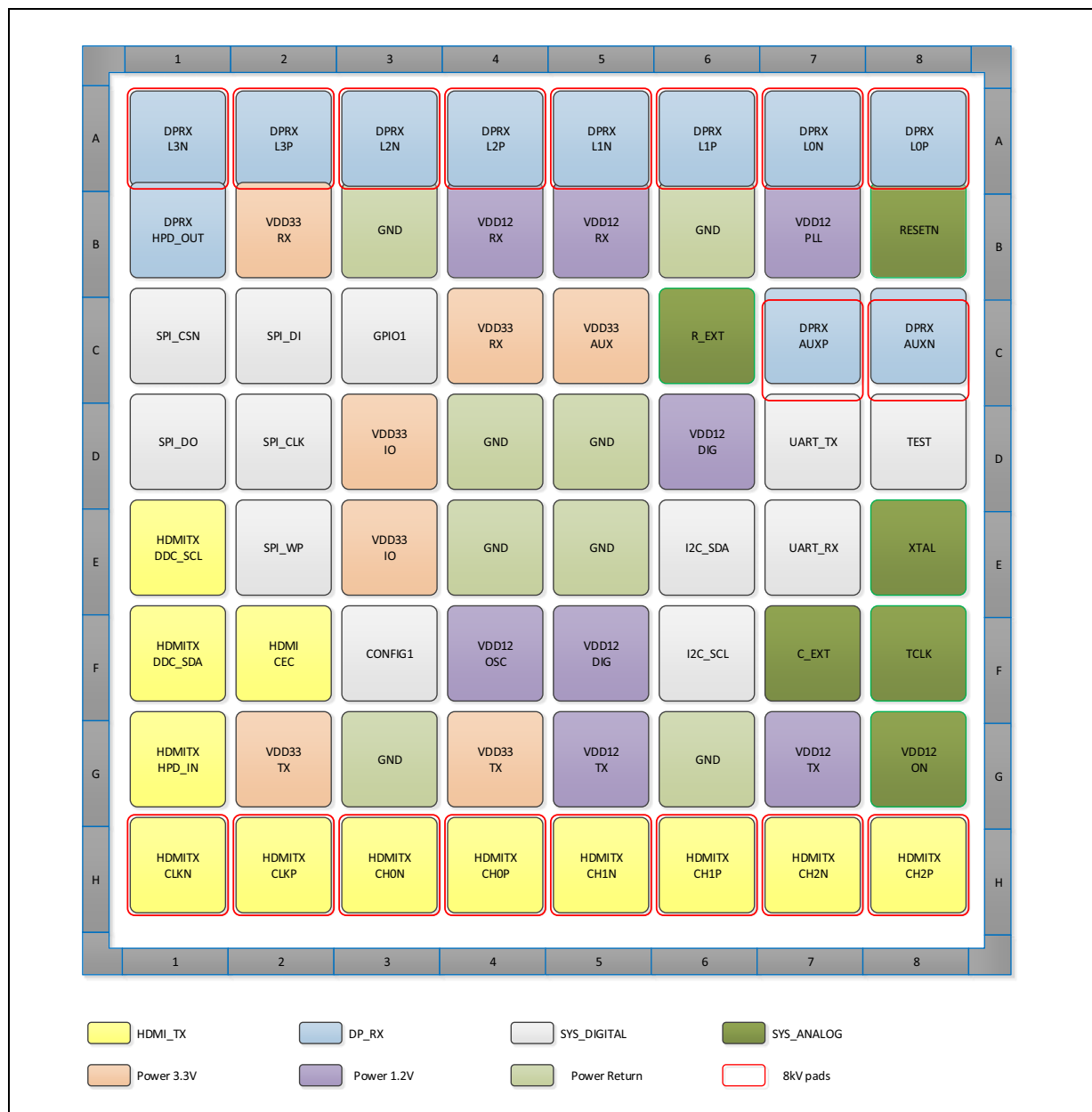
Figure 4. MCDP28x0 BGA diagram
