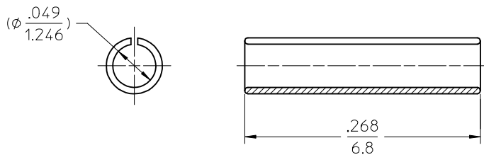
ALIGNMENT SLEEVE (ZIRCONIA CERAMIC)
