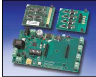
Digital LED Lighting Development Kit (DM330014)
