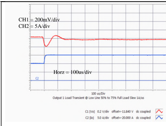
Vo=12V Typical output voltage transient response to load step from 50% to 75% of full load with output current slew rate of 1A/uS. (Cext = 200uF)
