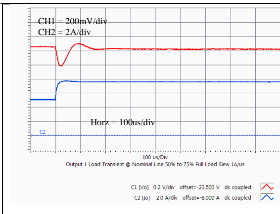
Vo=24V Typical output voltage transient response to load step from 50% to 75% of full load with output current slew rate of 1A/uS. (Cext = 22uF)
