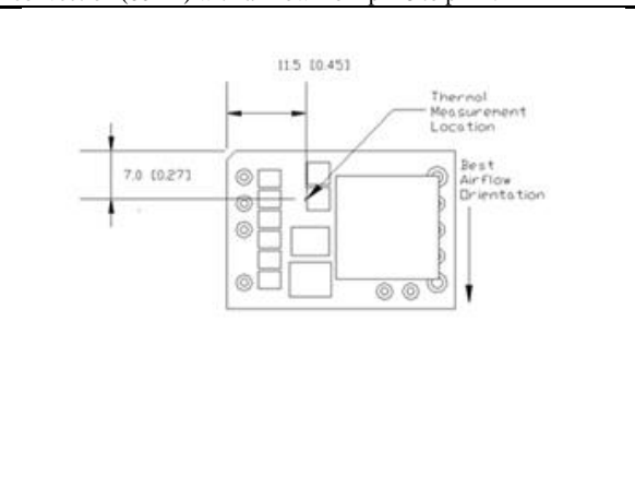
i6A4W010A033V thermal measurement location – top view
