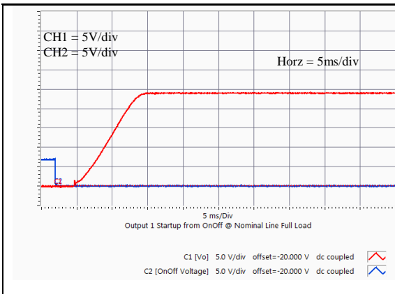
Vo=24V Typical startup characteristic from on/off at full load. Ch1 - output voltage, Ch2 – on/off signal
