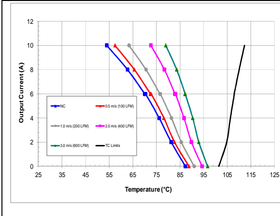
Vo=24V, Vin=36V preliminary maximum output current vs. ambient temperature at nominal input voltage for natural convection (60lfm) with airflow from pin 4 to pin 3.
