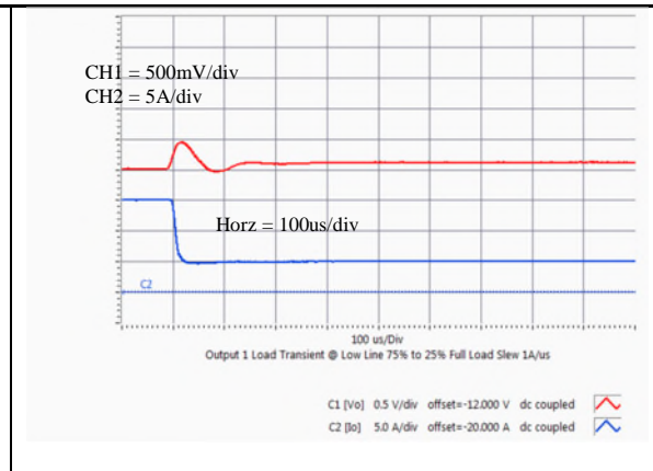
Vo=12V Typical output voltage transient response to load step from 75% to 25% of full load with output current slew rate of 1A/uS. (Cext = 200uF capacitor)
