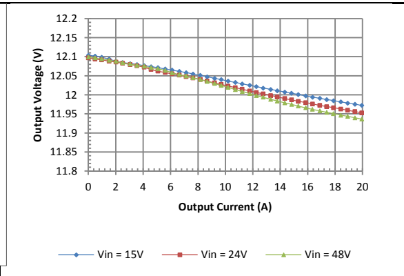
Vo=12V Typical load regulation
