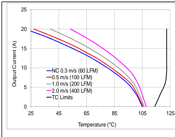
V_o=5V , V_{in}=36V preliminary maximum output current vs. ambient temperature at nominal input voltage for natural convection (60lfm) with airflow from pin 8 to pin 4.
