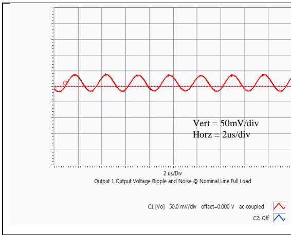
Vo=24V Typical Output Ripple at nominal Input voltage and full load at Ta=25 degrees
