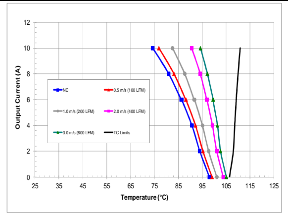
Vo=12V, Vin=24V preliminary maximum output current vs. ambient temperature at nominal input voltage for natural convection (60lfm) with airflow from pin 8 to pin 4.
