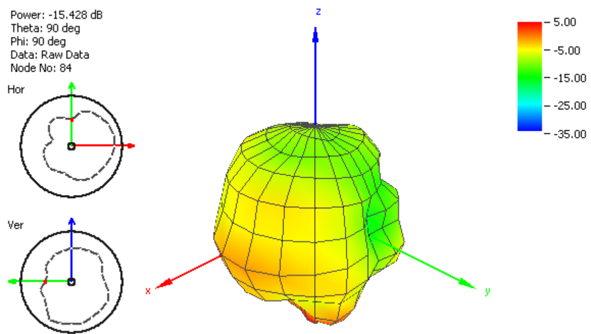
Figure 6. Radiation pattern at 915 MHz on a Piece of Road.
