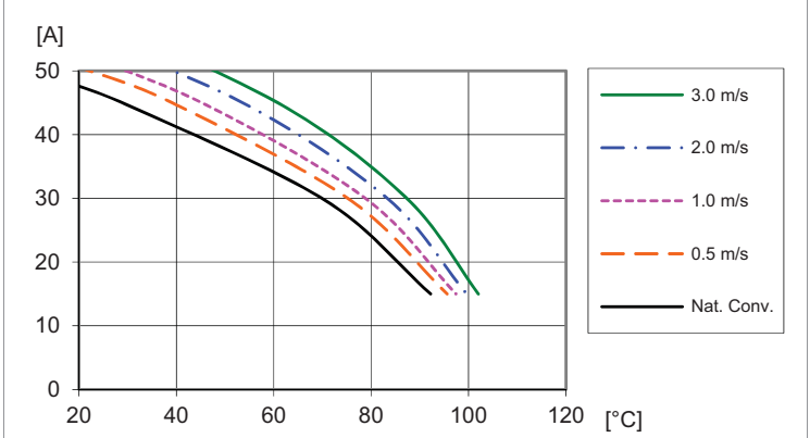
Output Current Derating, V_O = 3.3 V
