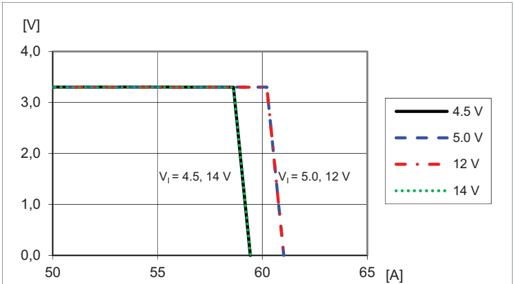
Current Limit Characteristics, V_O = 3.3 V
