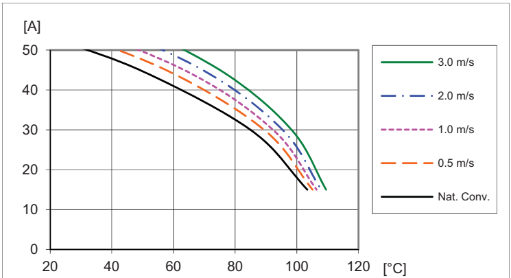
Output Current Derating, V_O = 1.0 V
