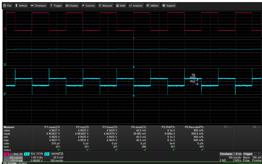
Figure 1: Using parameters and parameter math to measure load regulation
