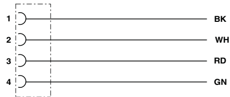
Contact assignment of 7/8" plugs/sockets, cable type 410
