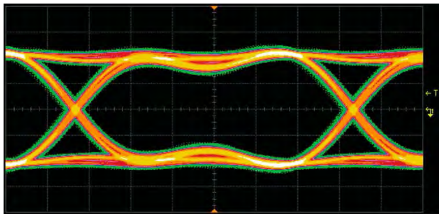
Fig 7. HDMI 2.0 TP1 eye diagram, PCB with PUSB3AB4
