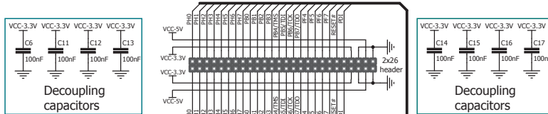
Figure 6-2: Pin headers
