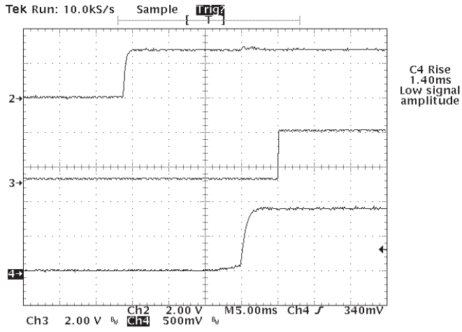
Figure 7: Control On/Off (Channel 2: Remote ON/OFF, Channel 3: Power Good Channel 4: Output Voltage)
