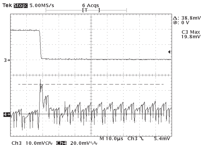
Figure 21: Transient Response 75 - 50% (Channel 3: Current load step at 5A/div, Channel 4: Output Voltage deviation)
