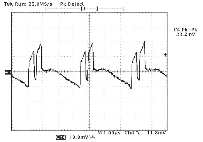
Figure 8: Typical Ripple and Noise
