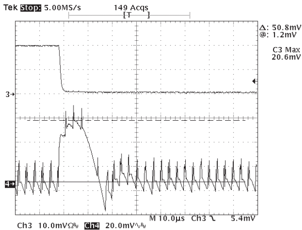
Figure 5: Transient Response 75 - 50% (Channel 3: Current load step at 5A/div, Channel 4: Output Voltage deviation)
