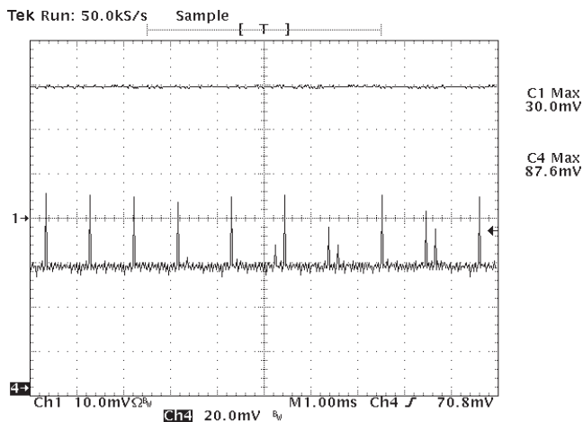
Figure 19: Short Circuit Characteristic (Channel 1: Output Current at 10A/div, Channel 4: Output Voltage)
