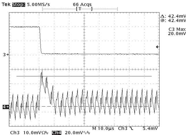
Figure 13: Transient Response 75 - 50% (Channel 3: Current load step at 5A/div, Channel 4: Output Voltage deviation)
