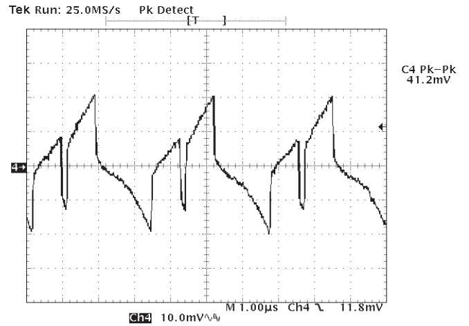
Figure 16: Typical Ripple and Noise
