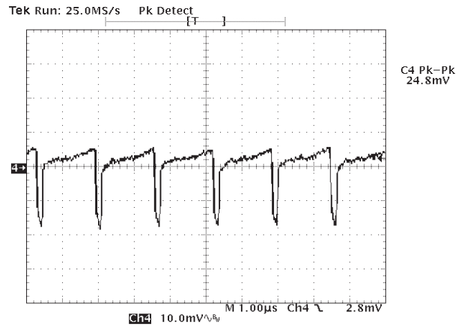
Figure 24: Typical Ripple and Noise
