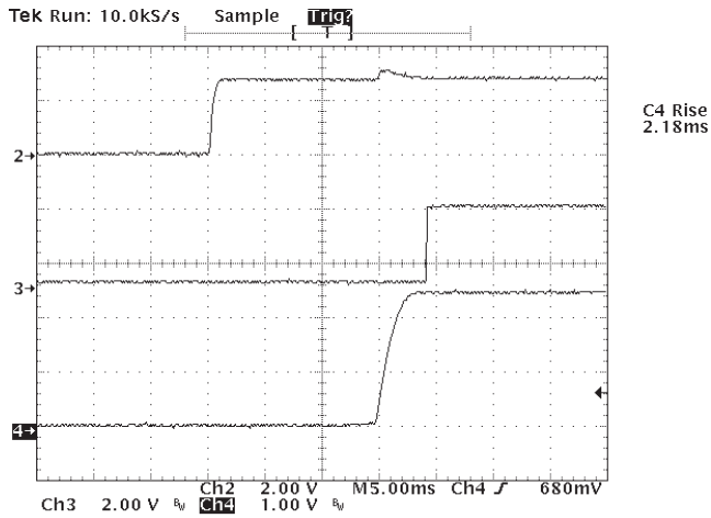
Figure 15: Control On/Off (Channel 2: Remote ON/OFF, Channel 3: Power Good Channel 4: Output Voltage)
