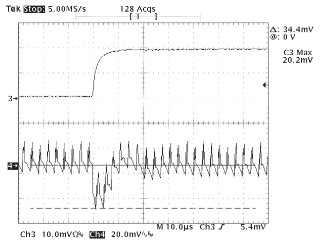
Figure 4: Transient Response 50-75% (Channel 3: Current load step at 5A/div, Channel 4: Output Voltage deviation)
