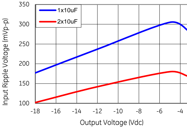
Figure 63. Input ripple voltage with 1x10 μF or 2x10 μF ceramic capacitors at the input (max load).
