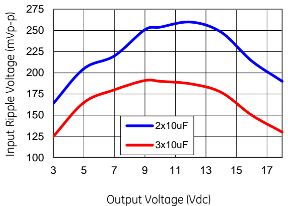
Figure 29. Input ripple voltage for various output voltages with 2x10 μF or 3x10 μF ceramic capacitors at the input (maximum load). Input voltage is 28V.
