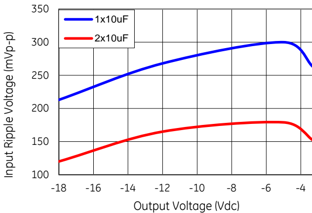
Figure 64. Input ripple voltage with 1x10 μF or 2x10 μF ceramic capacitors at the input (max load).
