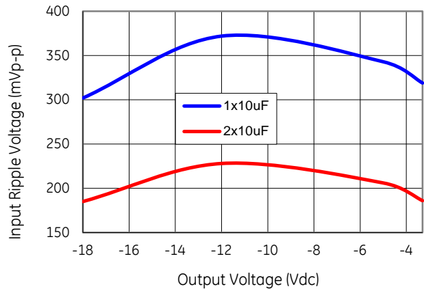
Figure 65. Input ripple voltage with 1x10 μF or 2x10 μF input ceramic capacitors (max load).
